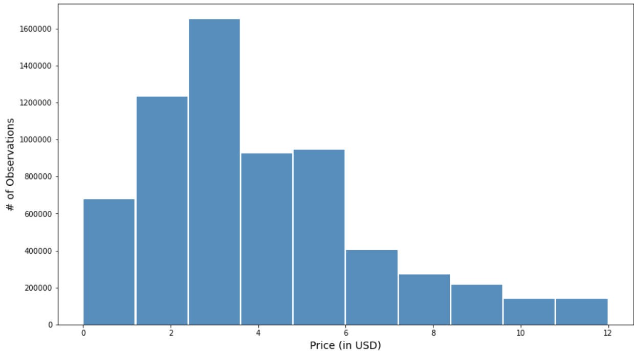
Histogram Price Distribution of Walmart Items
