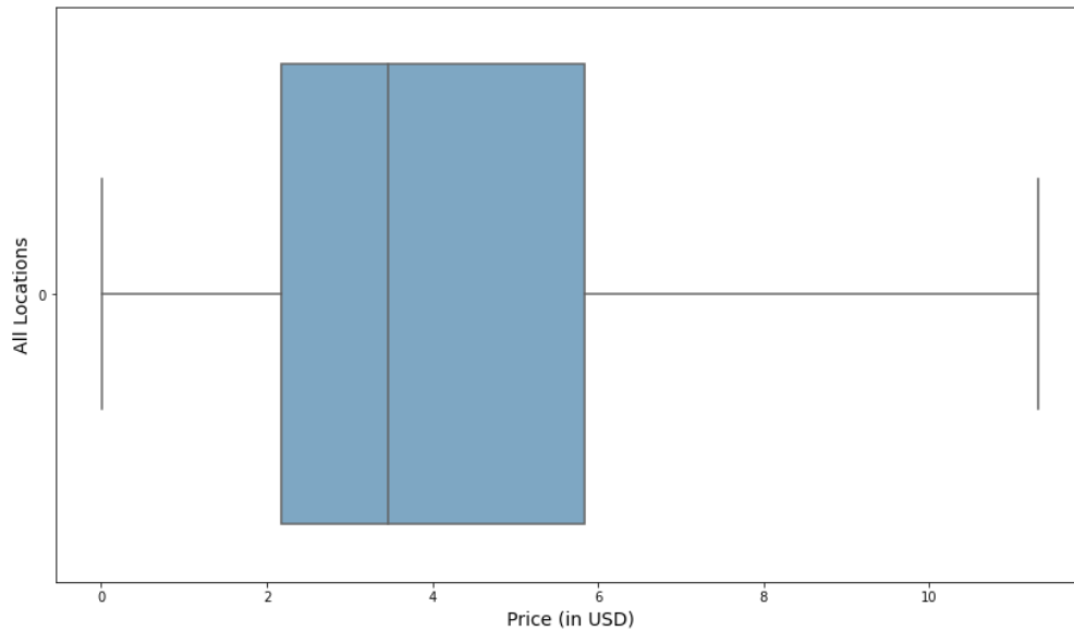
Boxplot Price Distribution of Walmart Items
